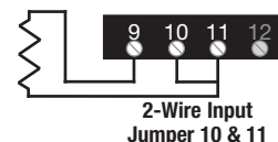
Two Wire RTD Input
