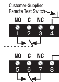
Relay Wiring APD 1430
