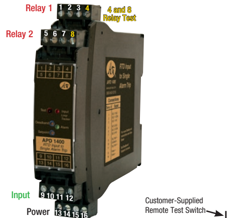
Relay Wiring APD 1400
