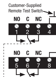
Relay Wiring APD 1400
