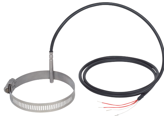
Fig. top: Model TR50-O with metal contact block
