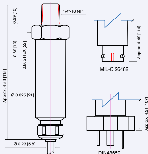
Ranges \leq 450 PSI
